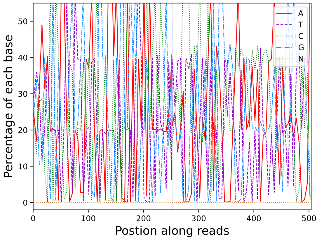
Base percentage along reads (R10409)
